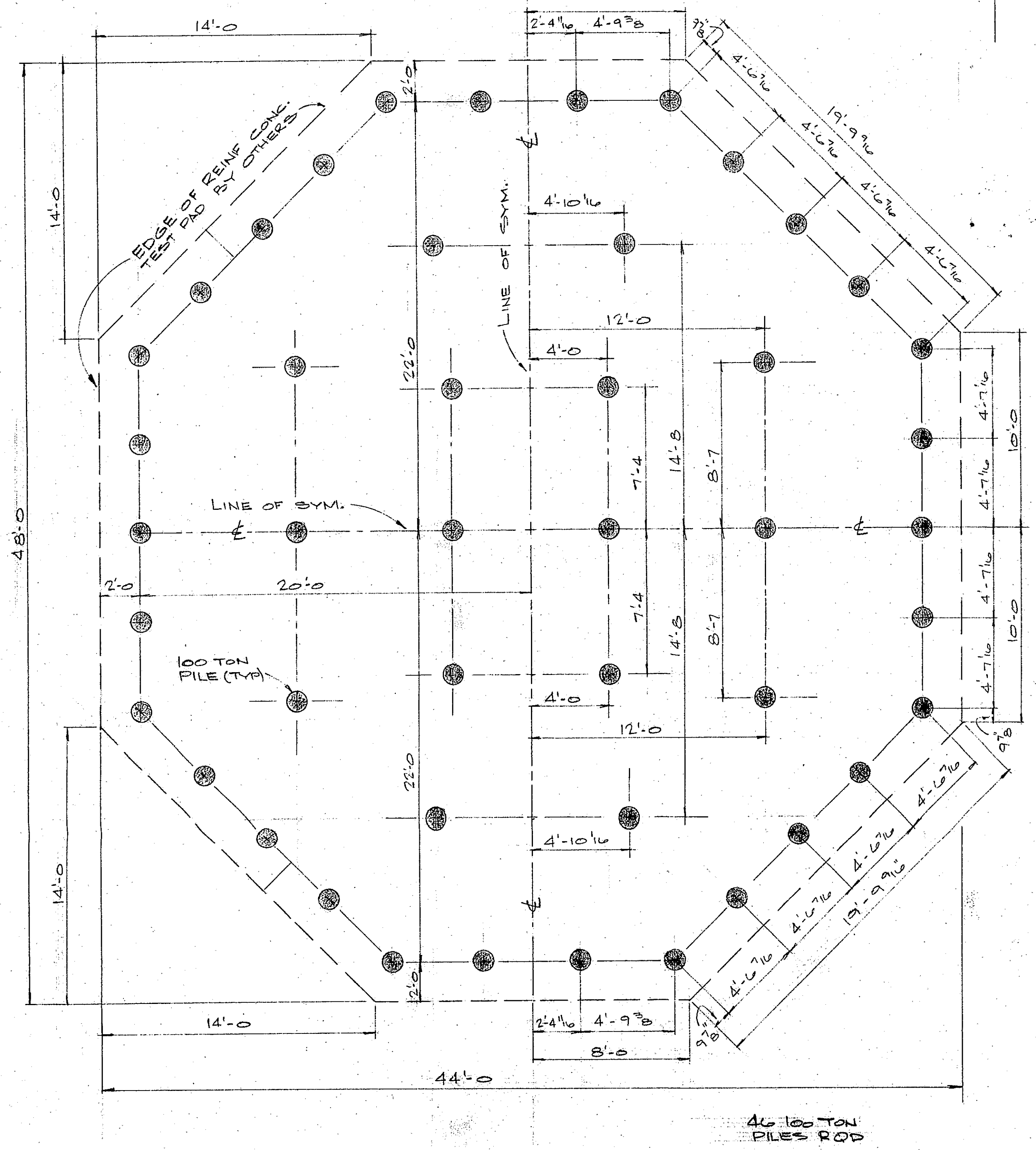
PILE PLAN AND GENERAL LAYOUT
